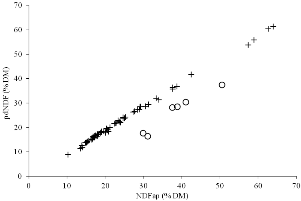
Figure 4.2 - Relationship between the contents of neutral detergent fiber corrected for ash and protein (NDFap) and potentially digestible neutral detergent fiber (pdNDF) in concentrate samples ( n = 65 ; \circ = concentrates containing fiber with lesser potential degradation; + = other concentrate feeds).
