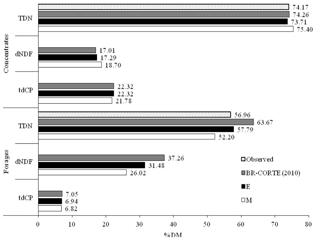
Figure 4.10 - Estimates of the truly digestible CP (tdCP), digestible NDF (dNDF) and the TDN content obtained by the sub-models adopted by the BR-CORTE (2010) and the meta-analytical (M) and empirical (E) approximations for growing and finishing cattle and TDN contents obtained from CQBAL 3.0 (forages, n = 16 ; concentrates, n = 8 ). The empirical and meta-analytical models considered intake of 22 g/kg body weight. For the meta-analytical model, a mean concentration was adopted of 12% CP and 14% iNDF in the diet. For the empirical and meta-analytical models applied to concentrates, corn silage was considered as the basal forage.
