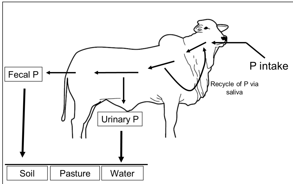
Scheme 13.2. Summary of the phosphorus cycle.
